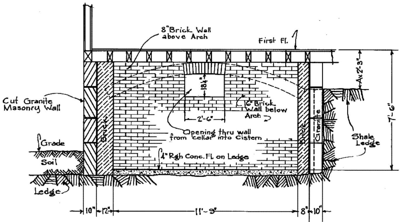
SECTION B-B
