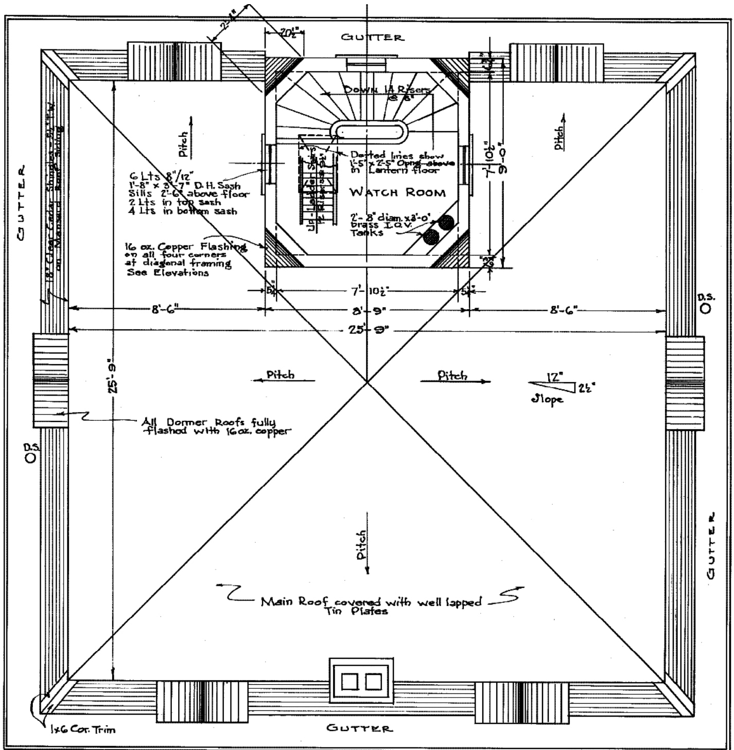
WATCH ROOM AND ROOF PLAN
